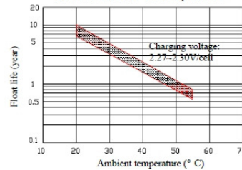
Float service life V'S temperature
