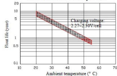
Float service life V'S temperature
