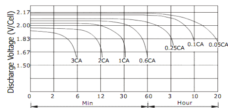
Discharge Characteristic (25°C)
