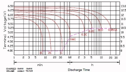
DISCHARGE CHARACTERISTICS AT 25° C(77° F)
