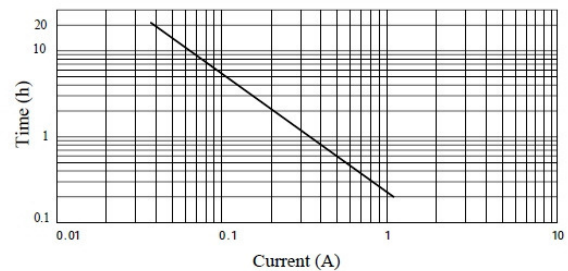
DISCHARGE CURRENT V'S TIME 25° C(77° F)
